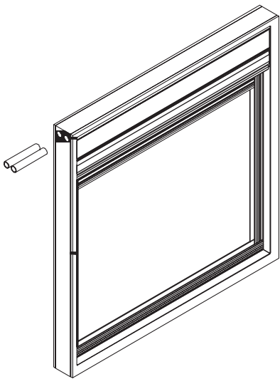
G removal of the silicon tubes
