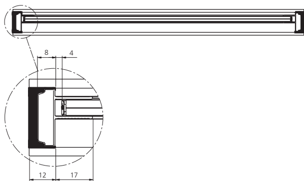
EXTRUDED "U" SPACER BAR 27X8 mm WITH 17 mm GUIDE PROJECTION
